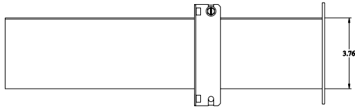
SIDE VIEW 3.76
